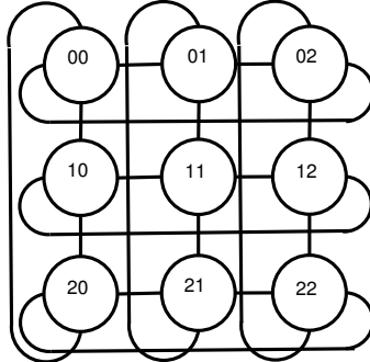
Fig. 14. 3-ary 2-cube network with endpoint numbering.
